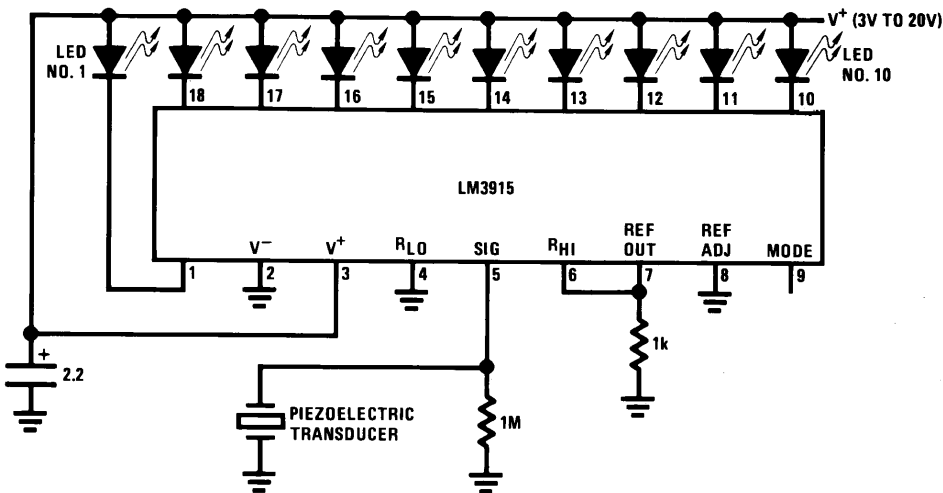
Figure 29. Vibration Meter
