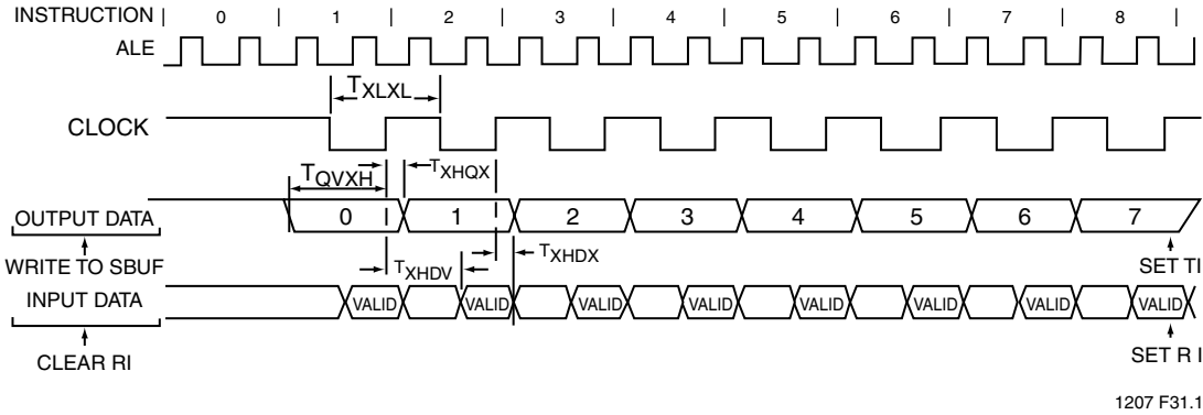
FIGURE 13-7: SHIFT REGISTER MODE TIMING WAVEFORMS
