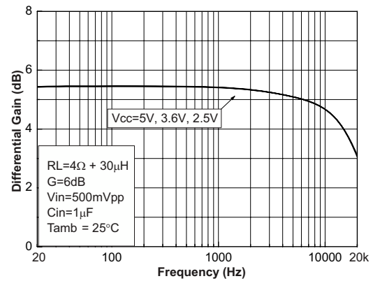
Figure 51. Gain vs. frequency at R_L = 4\ \Omega + 30\ \mu\text{H}
