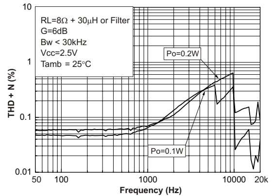
Figure 49. THD+N vs. frequency at R_L = 8\ \Omega + 30\ \mu\text{H} or filter, V_{CC} = 2.5\ \text{V}
