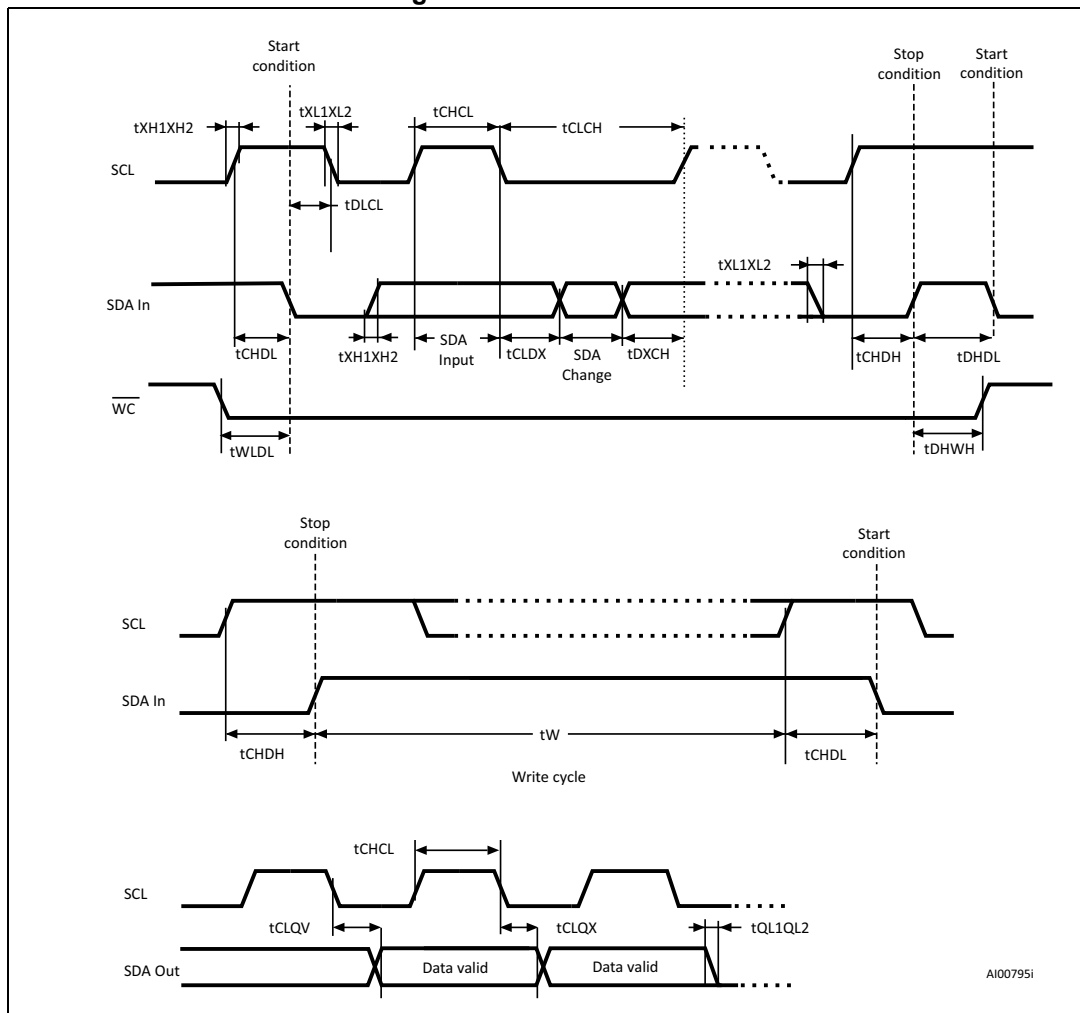
Figure 11. AC waveforms
