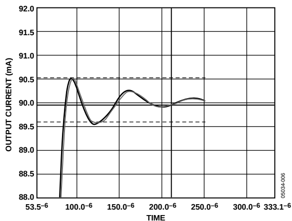
Figure 8. 1/4 to 3/4 Scale Settling Time ( V_{DD} = 3.6\text{ V} )
