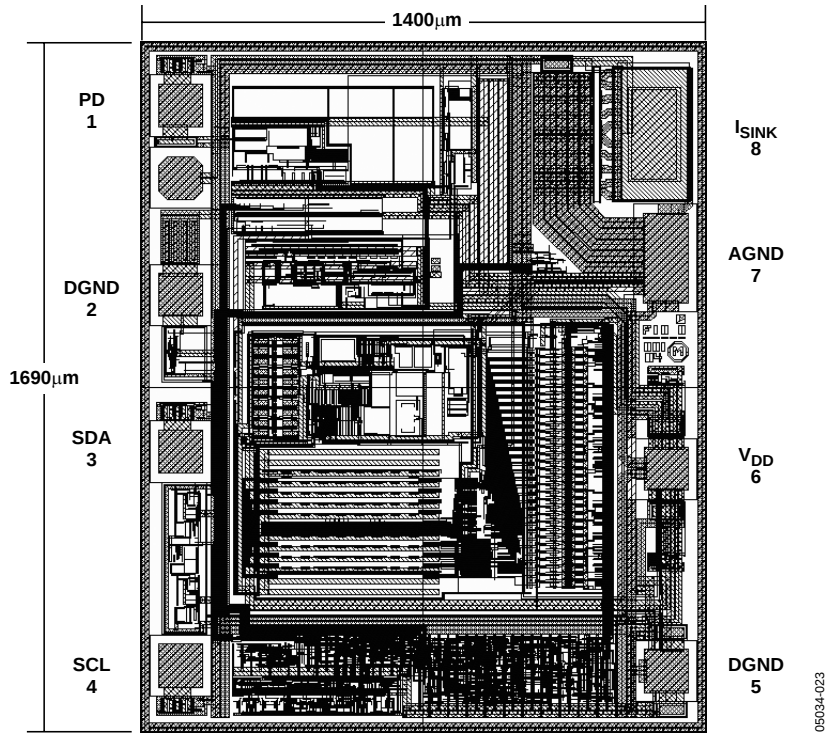
Figure 5. Metallization Photograph Dimensions shown in \mu\text{m} Contact Factory for Latest Dimensions
