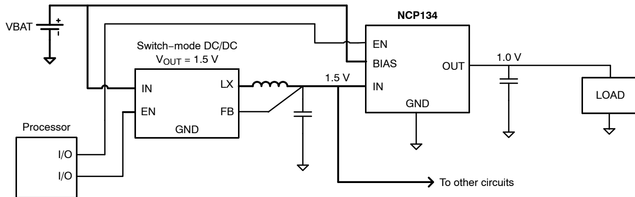
Figure 20. Typical Application: Low-Voltage DC/DC Post-Regulator with ON/OFF Functionality
