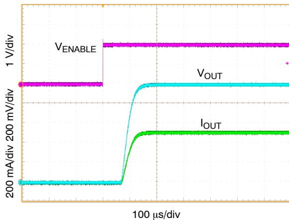
Figure 16. Enable Turn-on Response, Output Resistive Load 500\text{ mA} , C_{OUT} = 10\text{ }\mu\text{F}
