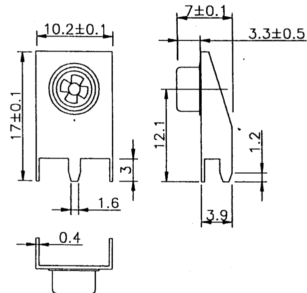
MALE CONTACT
