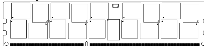
Figure 1: 240-Pin RDIMM (MO-269 R/C H0)
