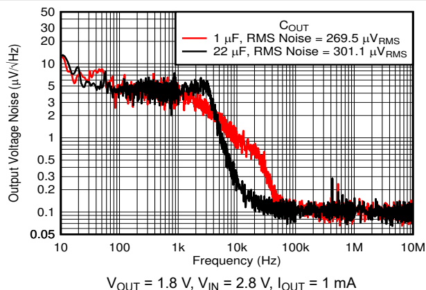
Figure 6-49. Output Noise vs Frequency and C_{OUT}
