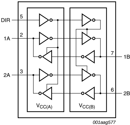
Fig 1. Logic symbol
