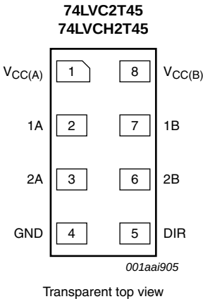
Fig 4. Pin configuration SOT833-1 (XSON8)
