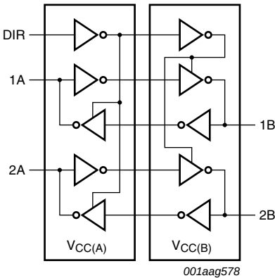
Fig 2. Logic diagram
