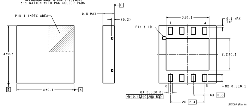
8-Lead LLP
