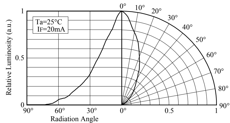
■ Directivity (NSPG320BS)
