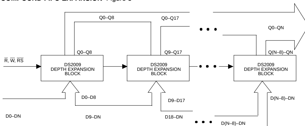
COMPOUND FIFO EXPANSION Figure 5
