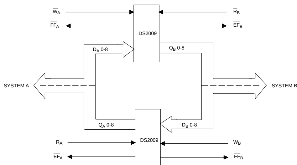
BIDIRECTIONAL FIFO APPLICATION Figure 6
