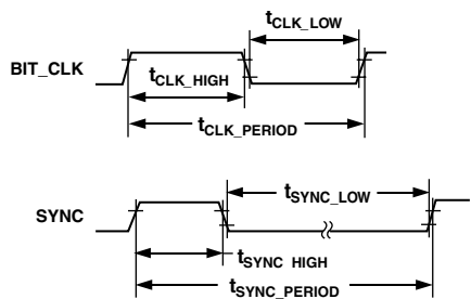
Figure 3. Clock Timing
