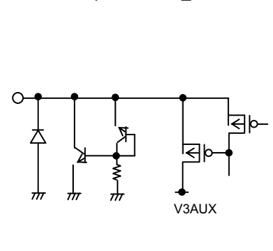
20pin&lt;V3AUX_IN&gt;
