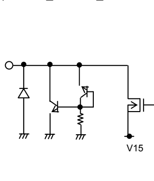
17,18pin&lt;V15_IN1,V15_IN2&gt;
