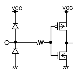
11pin&lt;CPPE#&gt;
