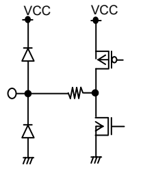
13pin&lt;PERST#_DELAY&gt;
