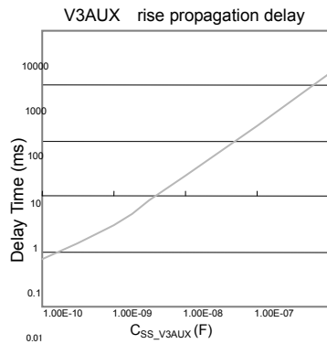
Fig.13 V3AUX rise propagation delay
