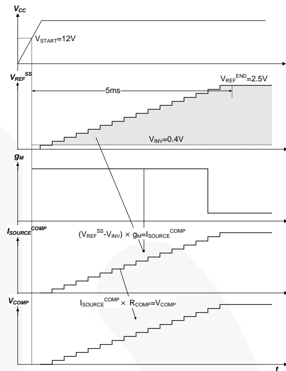
Figure 36. Soft-Start Sequence
