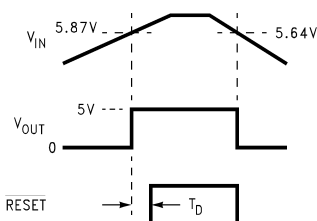
Figure 49. Timing Diagram
