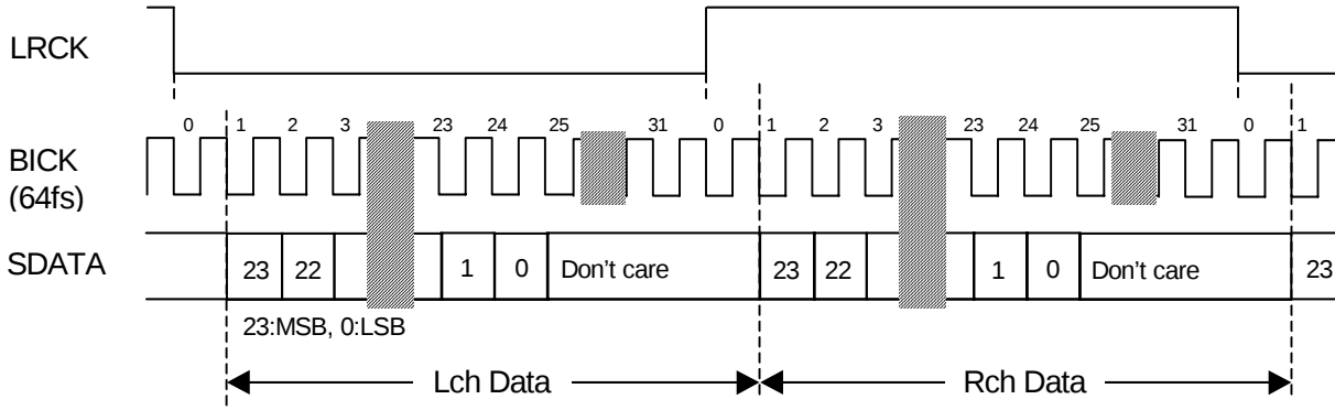
Figure 4. Mode 3 Timing
