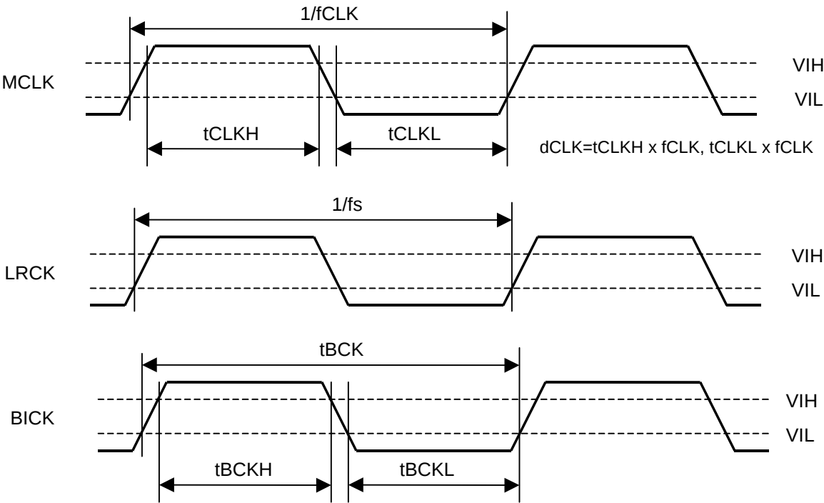
Clock Timing
