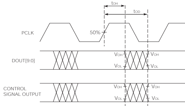
Figure 3-14: PCLK to Data & Control Signal Output Timing
