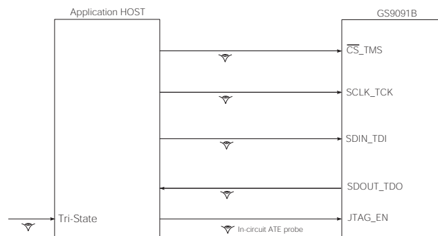
Figure 3-22: System JTAG
