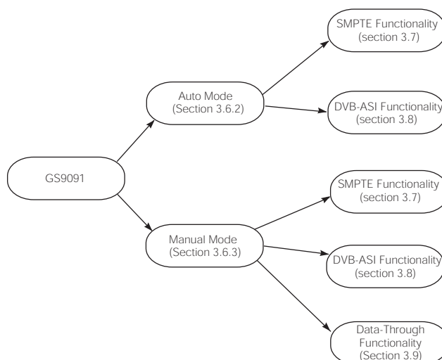
Figure 3-1: GS9091B's Modes of Operation
