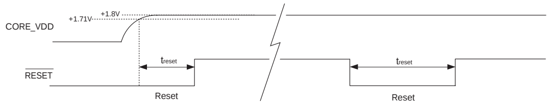
Figure 3-23: Reset pulse
