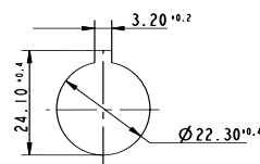
panel cut-out acc. to IEC 60947-5-1
