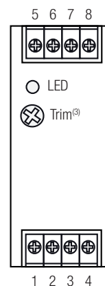
Pin Connections
