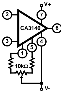
(B) IMPROVED RESOLUTION
