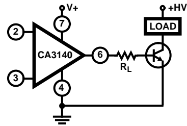
FIGURE 13. METHODS OF UTILIZING THE V_{CE(SAT)} SINKING CURRENT CAPABILITY OF THE CA3140 SERIES
