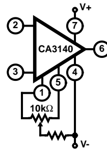
(C) SIMPLER IMPROVED RESOLUTION
