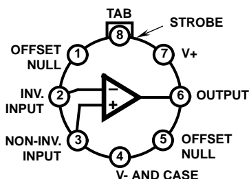
CA3140 (TO-5 STYLE CAN) TOP VIEW
