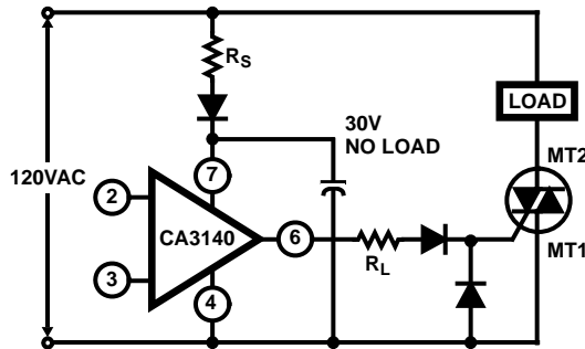
FIGURE 13. METHODS OF UTILIZING THE V_{CE(SAT)} SINKING CURRENT CAPABILITY OF THE CA3140 SERIES
