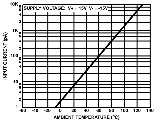
FIGURE 16. INPUT CURRENT vs AMBIENT TEMPERATURE
