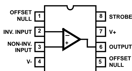
CA3140 (PDIP, SOIC) TOP VIEW
