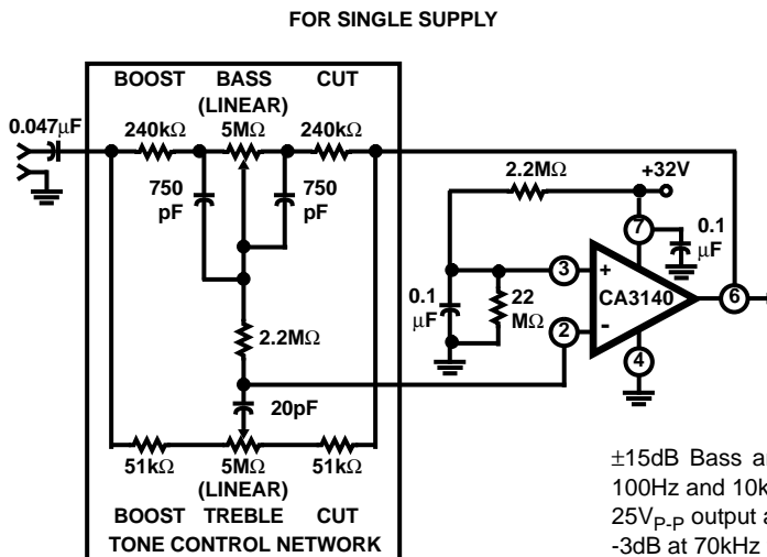
FIGURE 28. BAXANDALL TONE CONTROL CIRCUIT USING CA3140 SERIES
