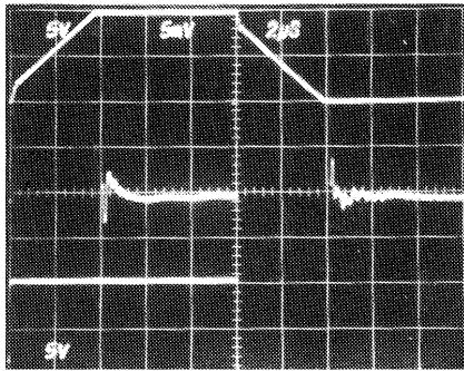
Top Trace: Output Signal; 5V/Div and 2μs/Div Center Trace: Difference of Input and Output Signals through Tektronix Amplifier 7A13; 5mV/Div and 2μs/Div Bottom Trace: Input Signal; 5V/Div and 2μs/Div
