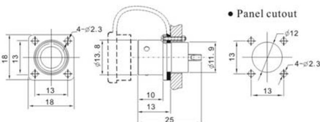
Square flange Mate with SF1210
