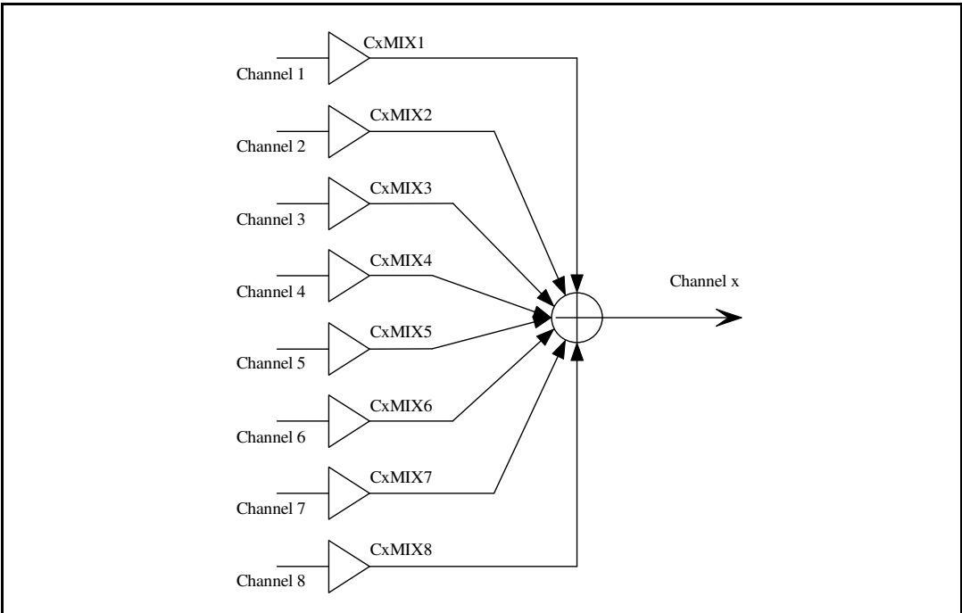
Figure 8. Channel mixer
