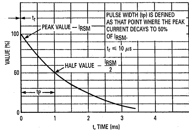
Figure 2. Pulse Waveform
