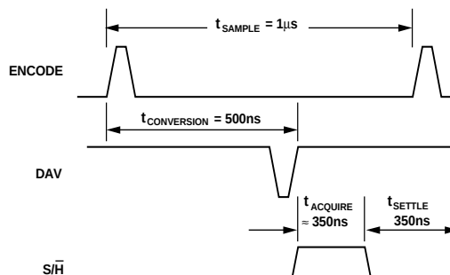
Figure 15. AD671 to Discrete SHA Timing Diagram
