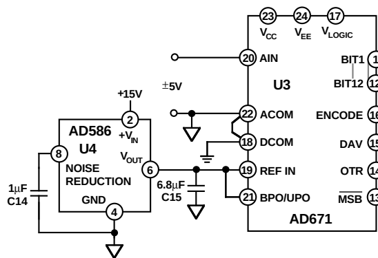
Figure 5. AD586 as Reference Input for AD671
