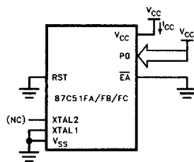
Figure 9. I_{CC} Test Condition, Power Down Mode. V_{CC} = 2.0V to 5.5V .
