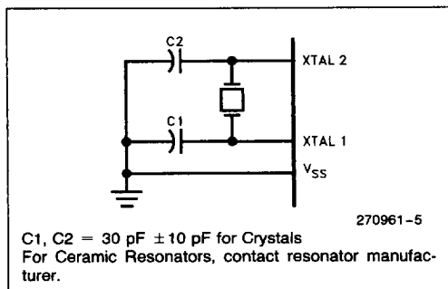
Figure 4. Oscillator Connections
