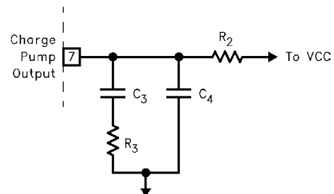
TYPICAL LOOP FILTER
