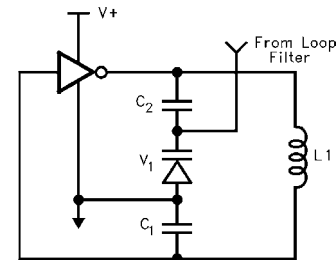
COLPITTS OSCILLATOR
