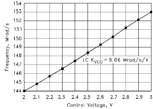
FOOSC vs VC, LC VCO
