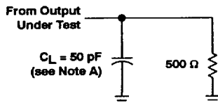
LOAD CIRCUIT
