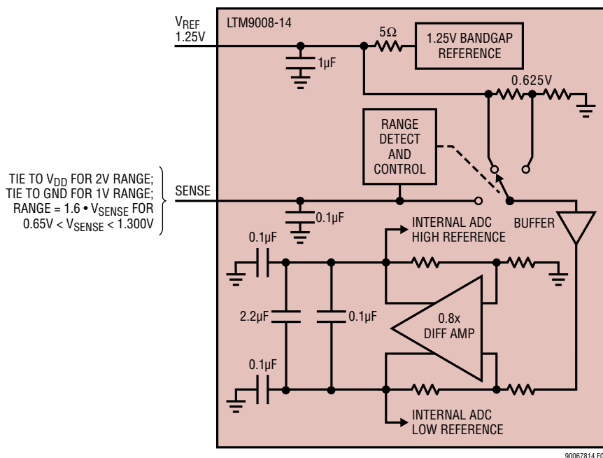
Figure 8. Reference Circuit
