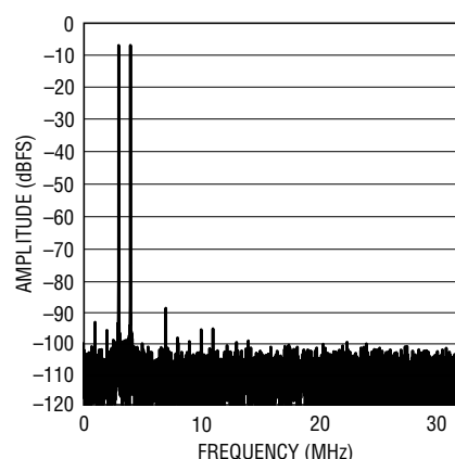
LTM9008-14, 65Msps, 2-Tone FFT, f_{IN} = 70 MHz and 75MHz
