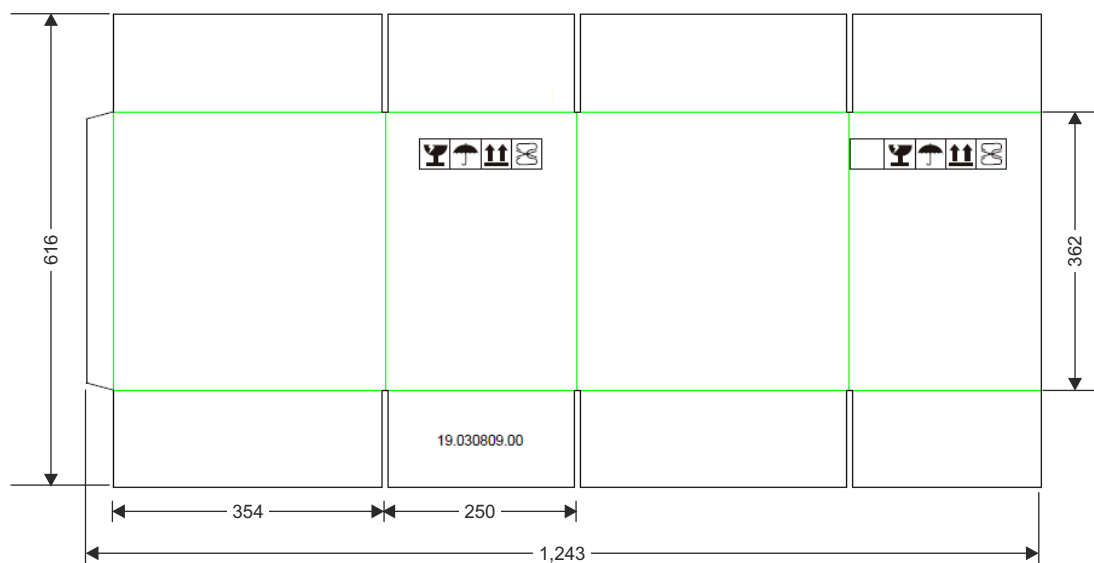
Figure 12-5. Shipping Box
