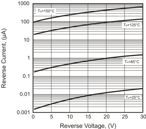
Fig.2 - Leakage Current
