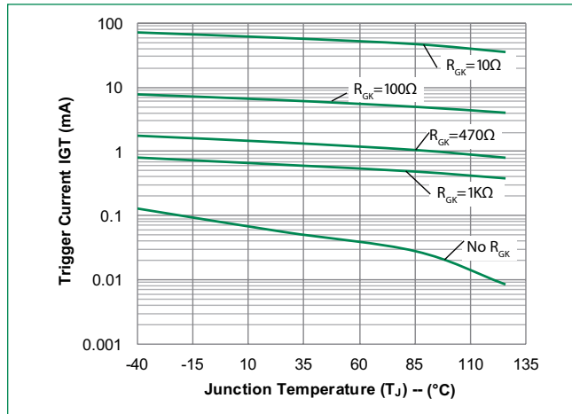
Figure 7: Typical DC Gate Trigger Current with R_{GK} vs. Junction Temperature for Sx02xS
