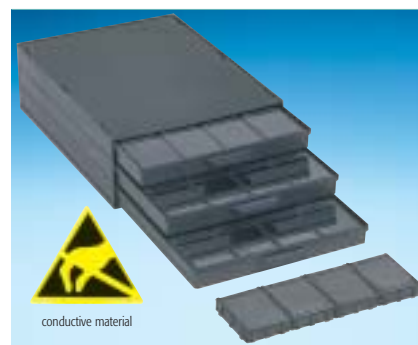
Art. No. SMD cabinet A 1-4 ESD 16 Cabinet with 3 drawers incl.
