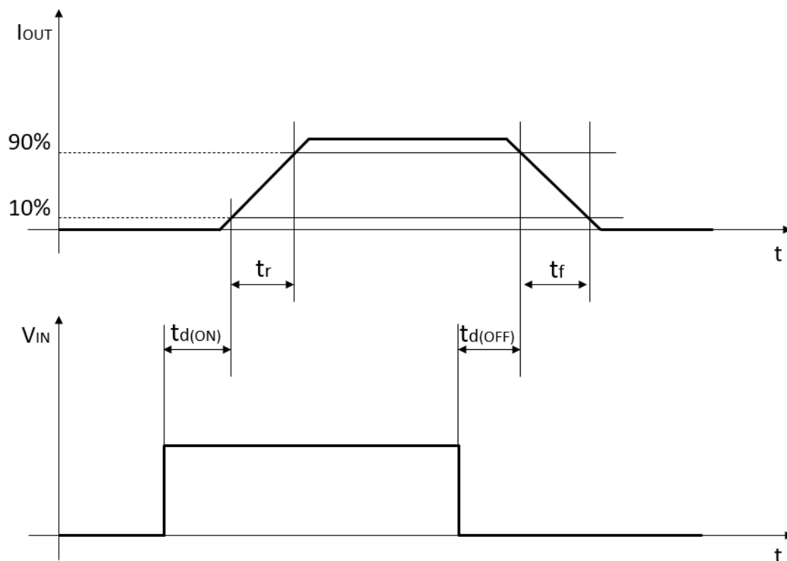
Figure 6. Switching parameter test conditions
