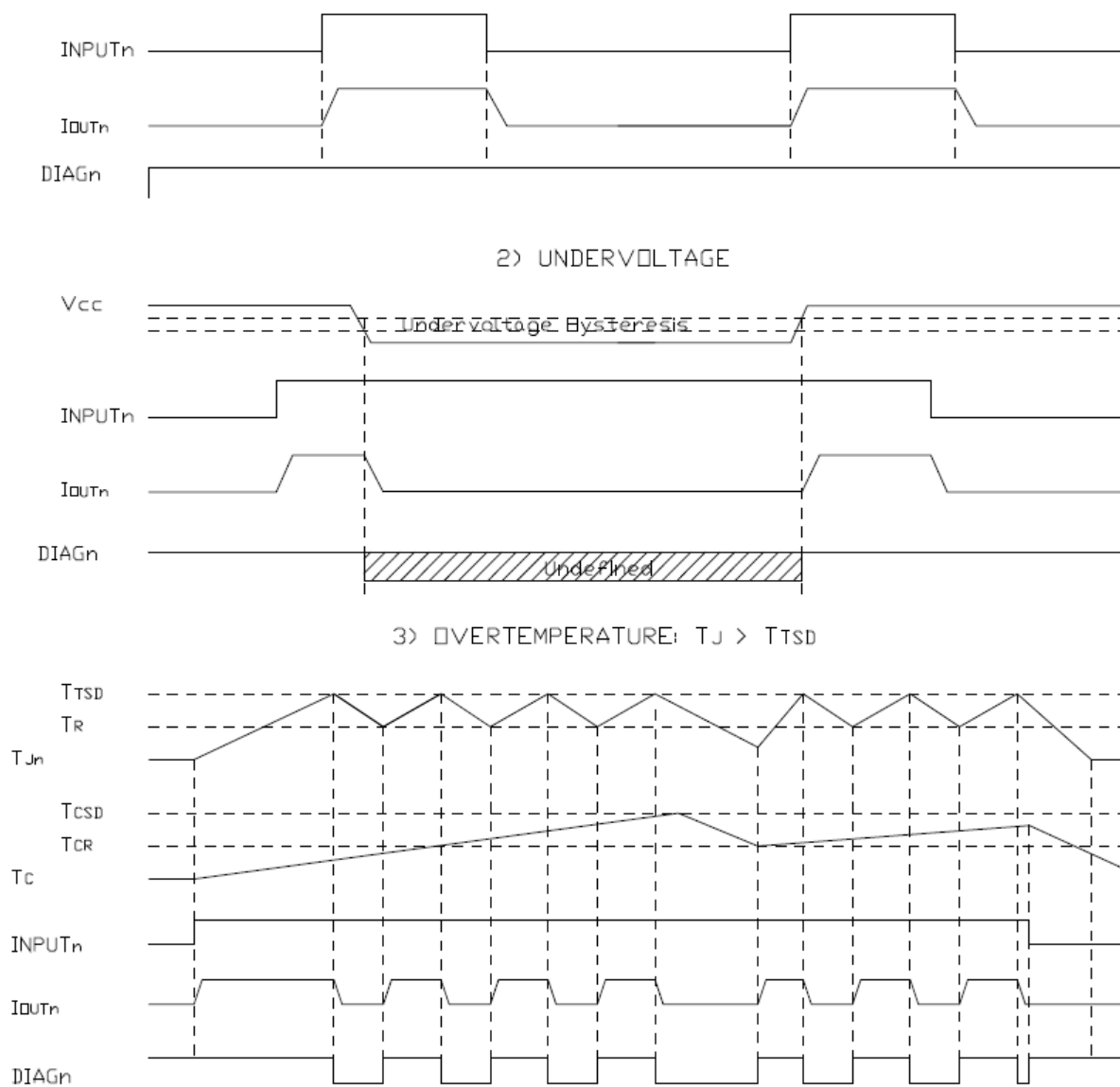
Figure 4. Switching waveforms
