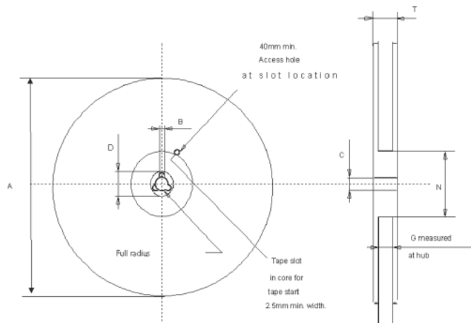
Figure 18. PowerSSO-12™ tape and reel shipment (suffix “TR”)
