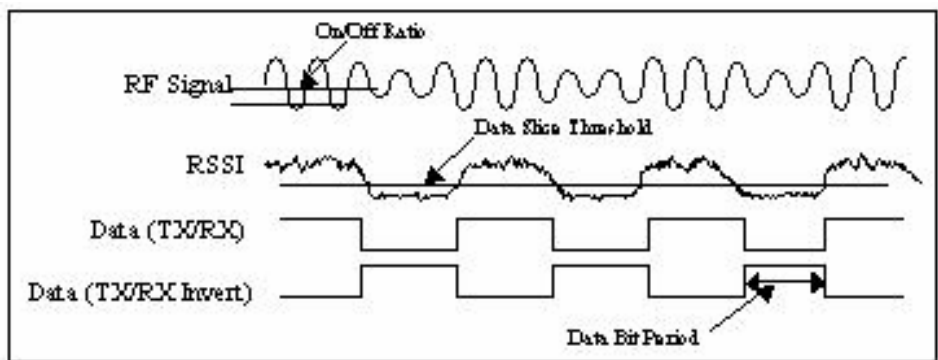
Figure 7: Received Waveform
