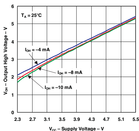
Figure 10. Output High Voltage vs Supply Voltage (P7-P1)
