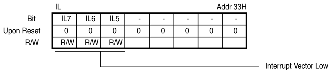
Figure 57. Interrupt Vector Low Register
