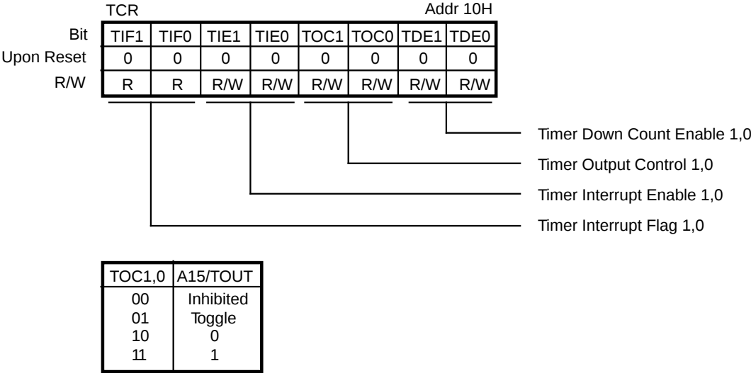
Figure 44. Timer Control Register
