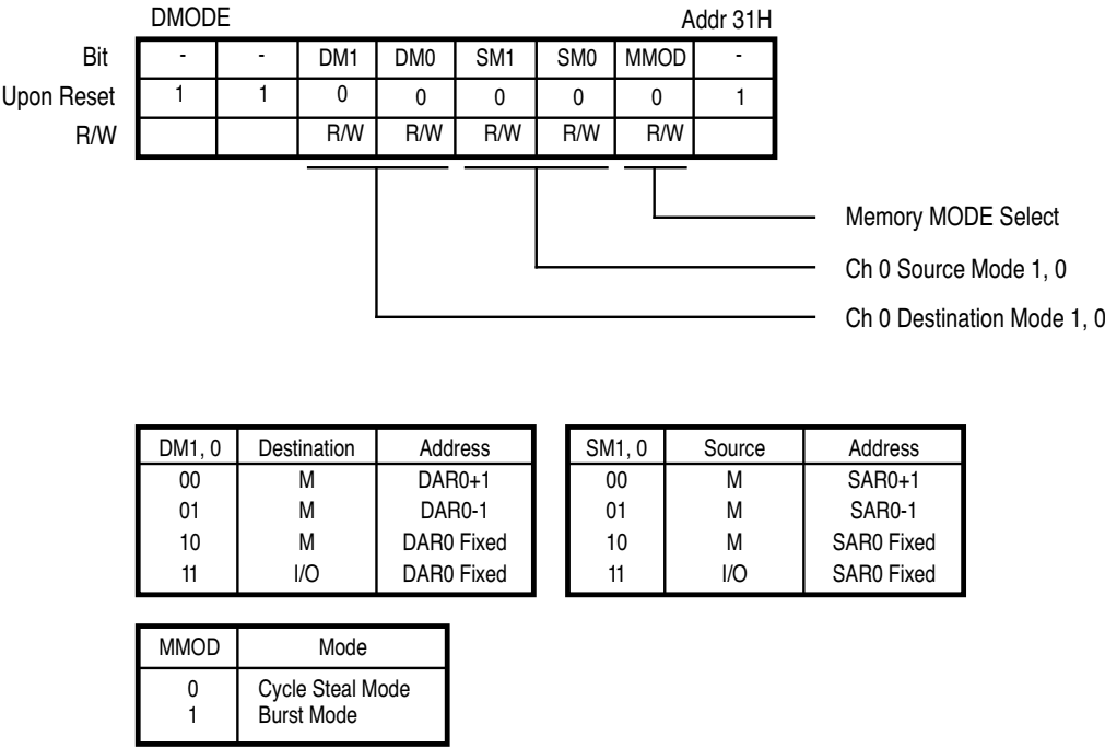
Figure 55. DMA Mode Registers
