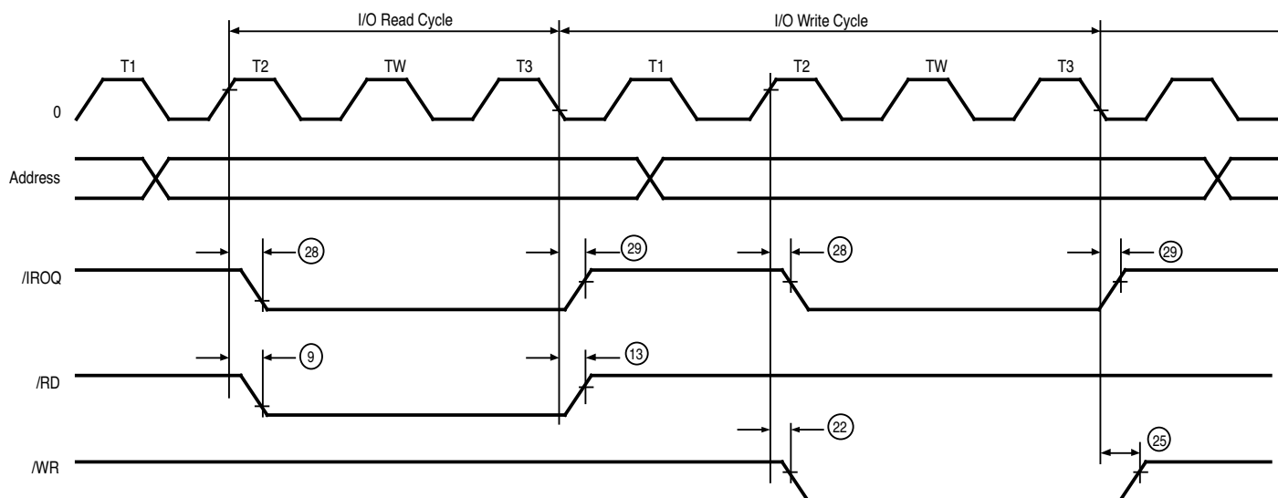
Figure 6. CPU Timing
