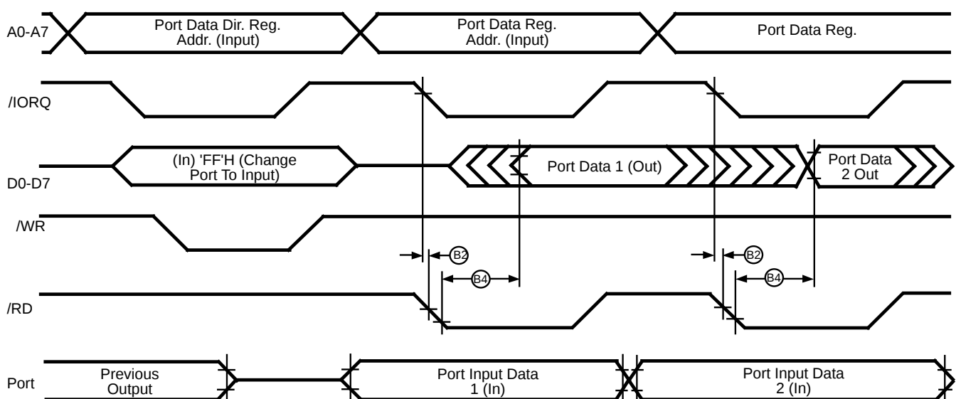
Figure 15. PORT Timing
