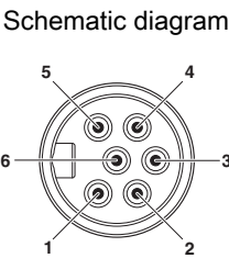
Pin assignment, plug, 7/8"-16UNF, 6-pos., view of male side
