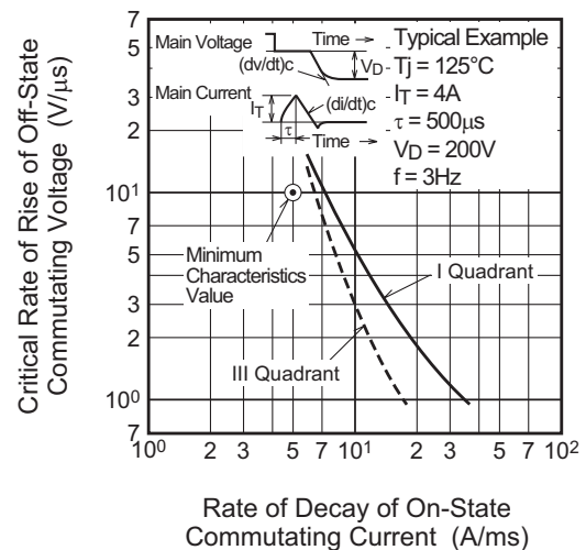
Commutation Characteristics ( T_j=125^\circ\text{C} )
