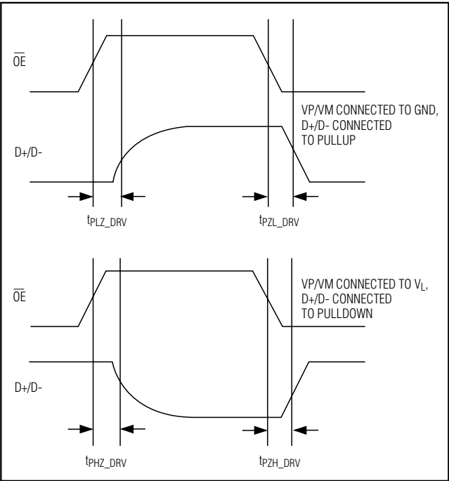
Figure 3. Driver Enable and Disable Timing
