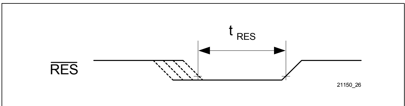
Figure 74 Reset Signal \overline{\text{RES}}
