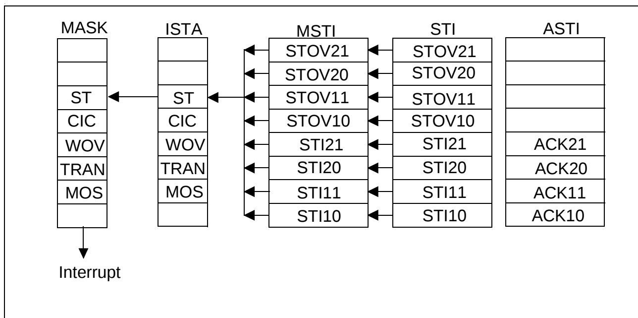
Figure 49 Interrupt Structure of the Synchronous Data Transfer
