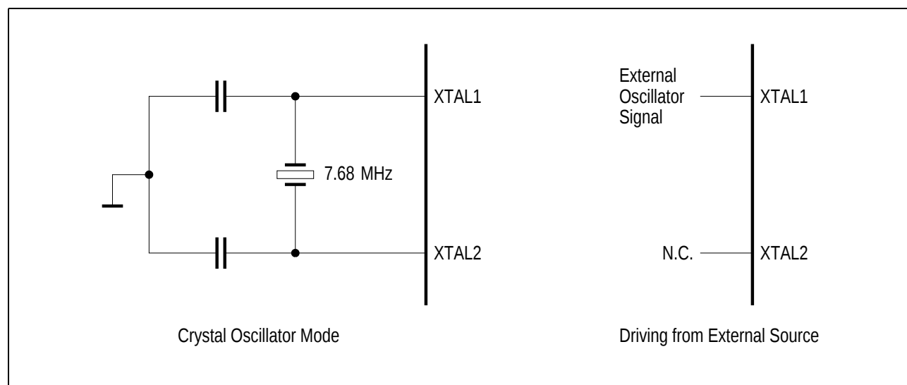
Figure 68 Oscillator Circuits
