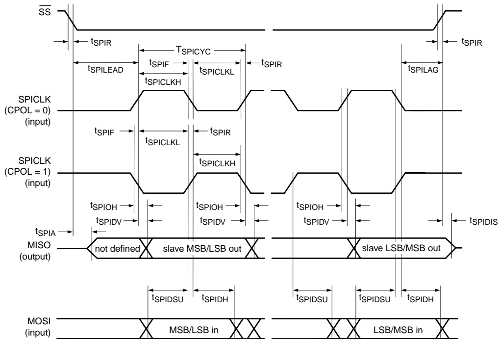
Fig 26. SPI slave timing (CPHA = 1)
