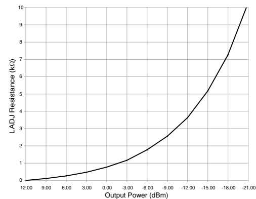
Figure 5: Output Power vs. LADJ Resistance
