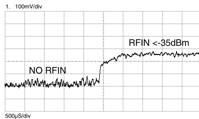
Figure 12: RSSI Response Time
