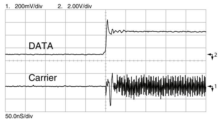
Figure 13: TX Modulation Delay
