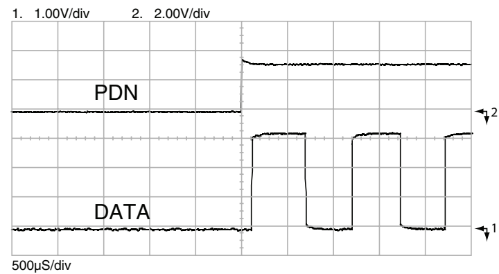
Figure 11: RX Turn-On Time from PDN
