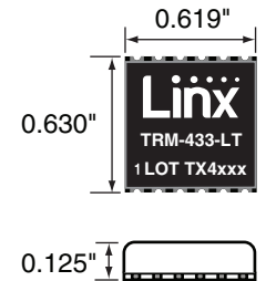
Figure 1: Package Dimensions
