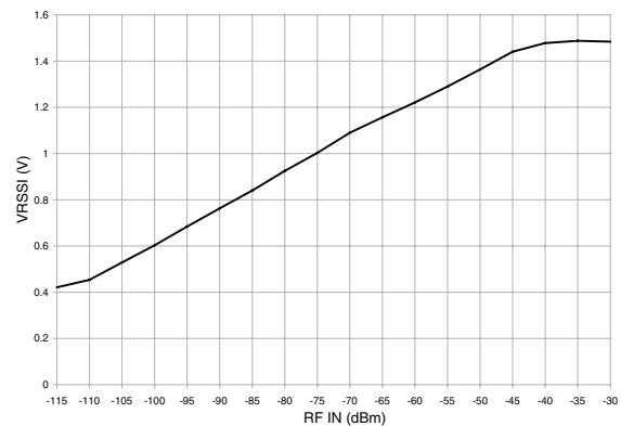
Figure 7: RSSI Curve
