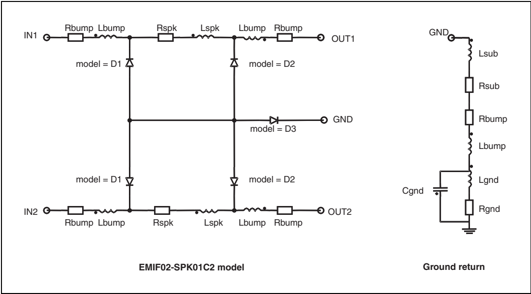
Figure 9. Aplac model
