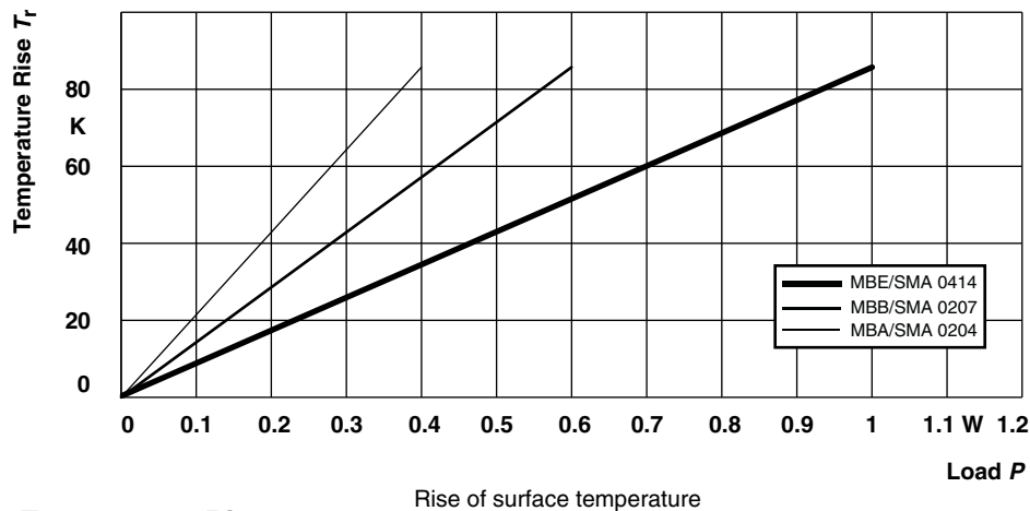
Temperature Rise
