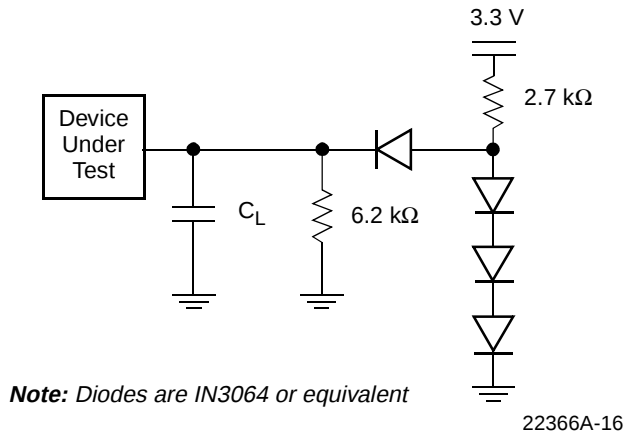
Figure 11. Test Setup
