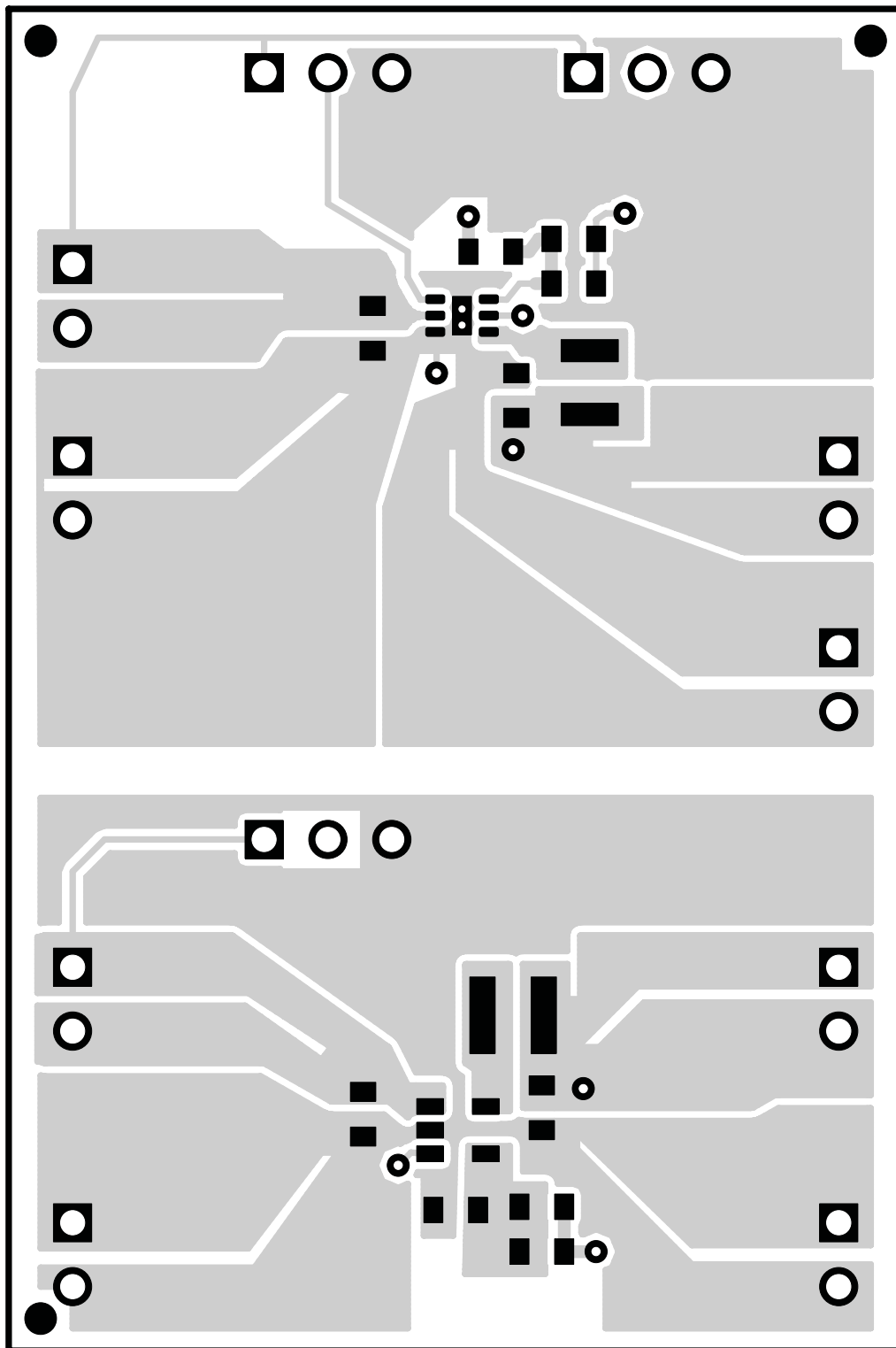
Figure 10. Top Layer Routing
