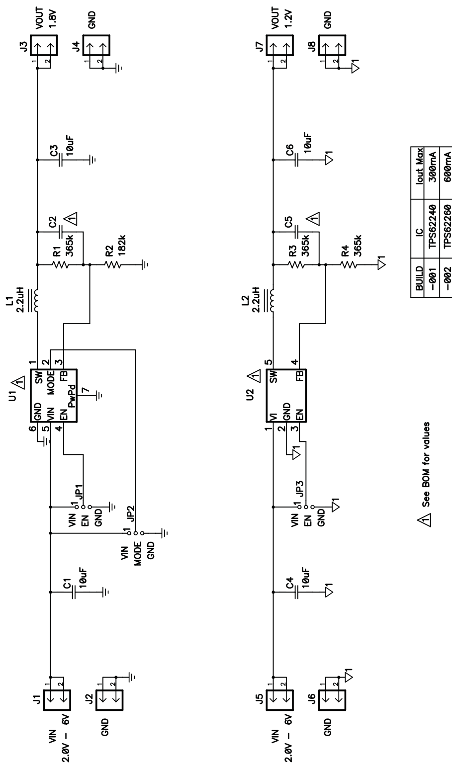
Figure 12. TPS622x0EVM-229 Schematic
