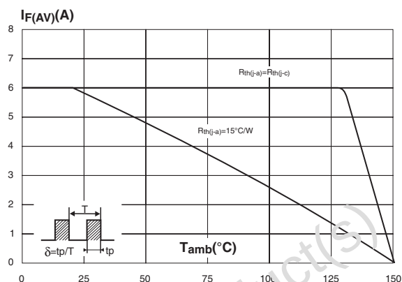
Figure 2: Average current versus ambient temperature ( \delta = 0.5 )
