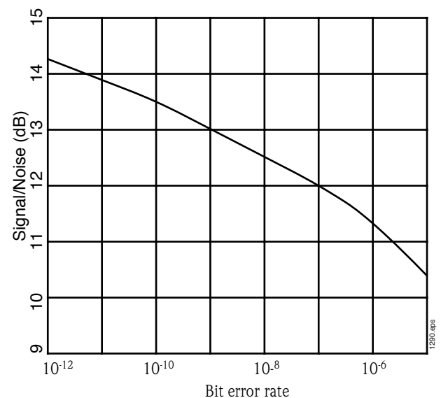
Figure 24. BER versus signal-to-noise ratio.
