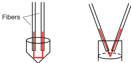
Figure 32. Liquid level and pressure sensors with optical fiber interfaces.
