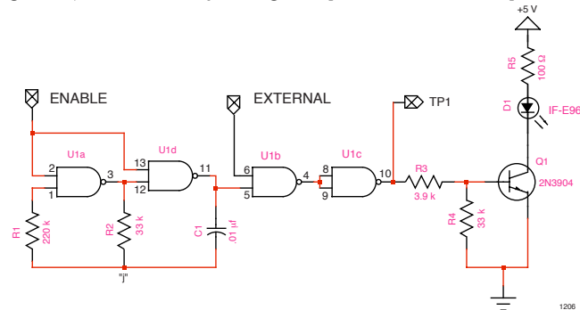
Figure 38. Transmitter circuit diagram.
